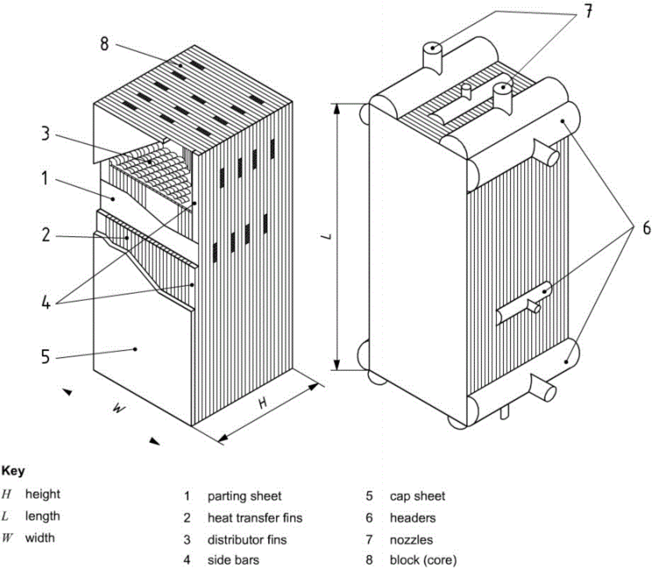
Figure 2 — Typical brazed aluminium plate-fin heat exchanger and components
