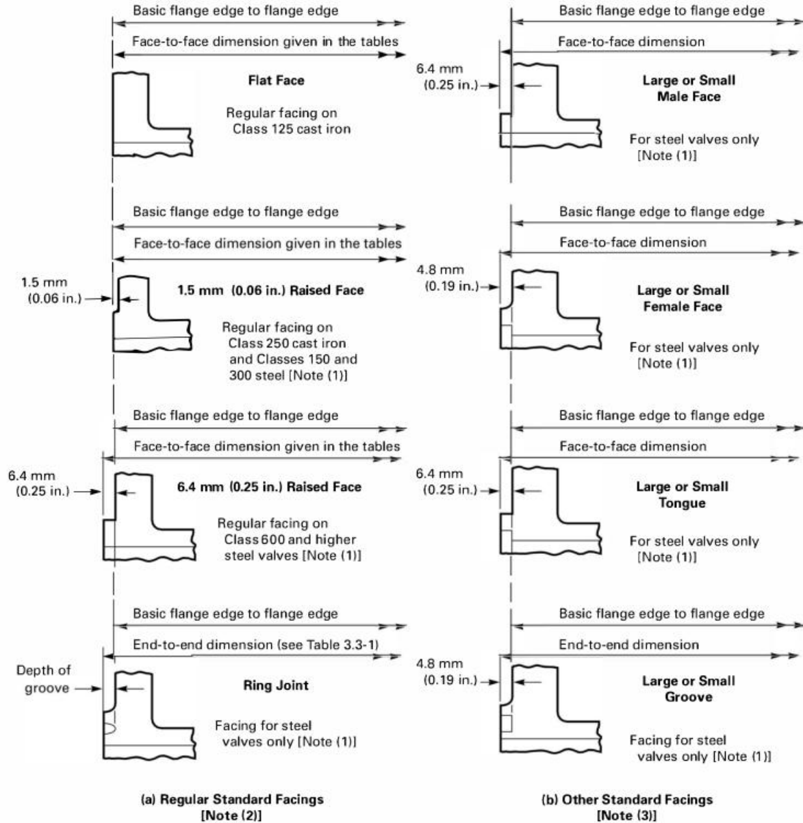
Figure 2.3.1-1 Flange Facings and Their Relationships
