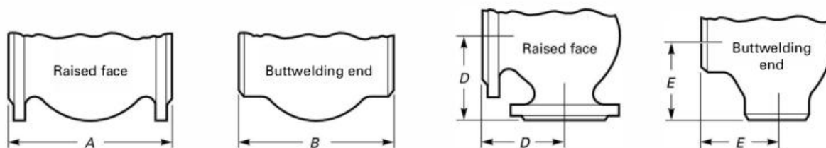
(22) Table 1.5-2 Class 900 Steel Flanged and Butt welding End Valves, Face-to-Face and End-to-End Dimensions
