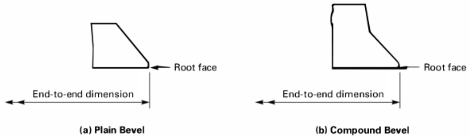
Figure 2.4-1 Welding Ends
